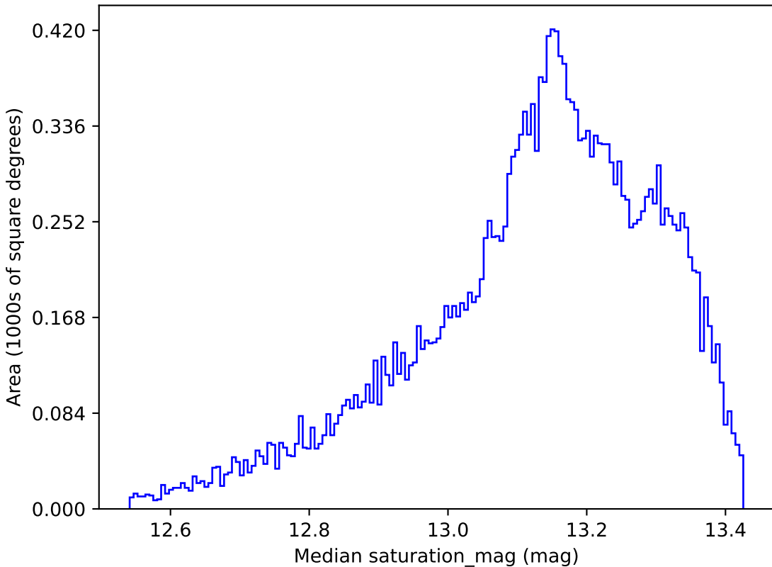
noroll_v3.4_10yrs All sky y band: Median saturation_mag
