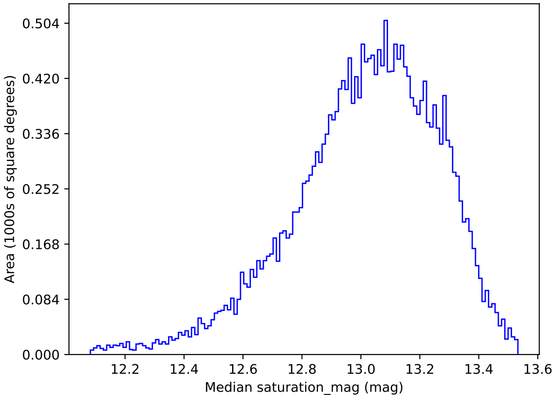
noroll_v3.4_10yrs All sky u band: Median saturation_mag
