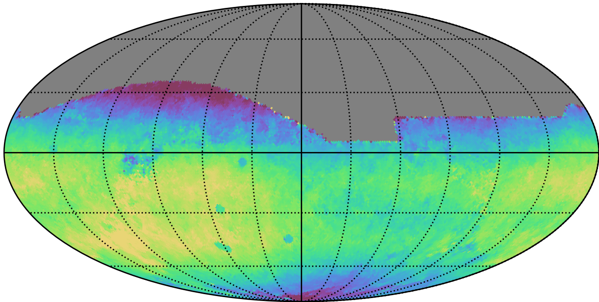
noroll_v3.4_10yrs All sky r band: Median saturation_mag
