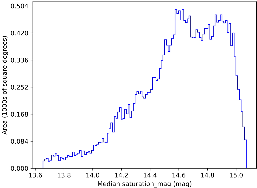
noroll_v3.4_10yrs All sky r band: Median saturation_mag
