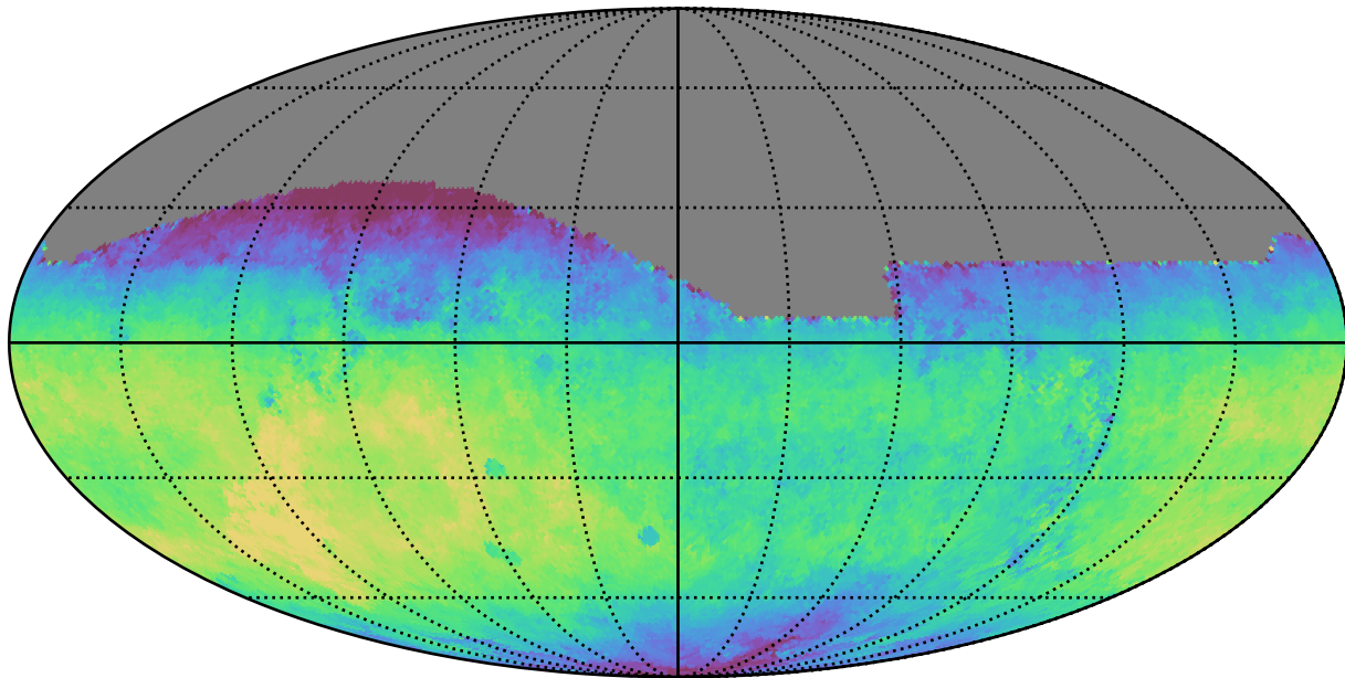
noroll_v3.4_10yrs All sky i band: Median saturation_mag
