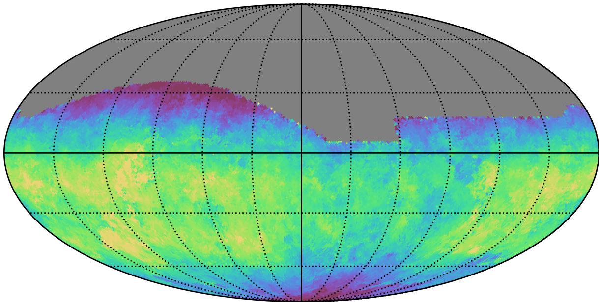
noroll_v3.4_10yrs All sky g band: Median saturation_mag
