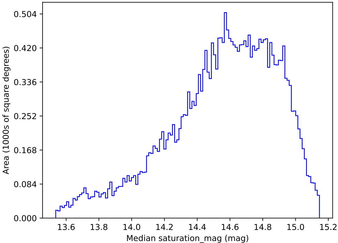
noroll_v3.4_10yrs All sky g band: Median saturation_mag
