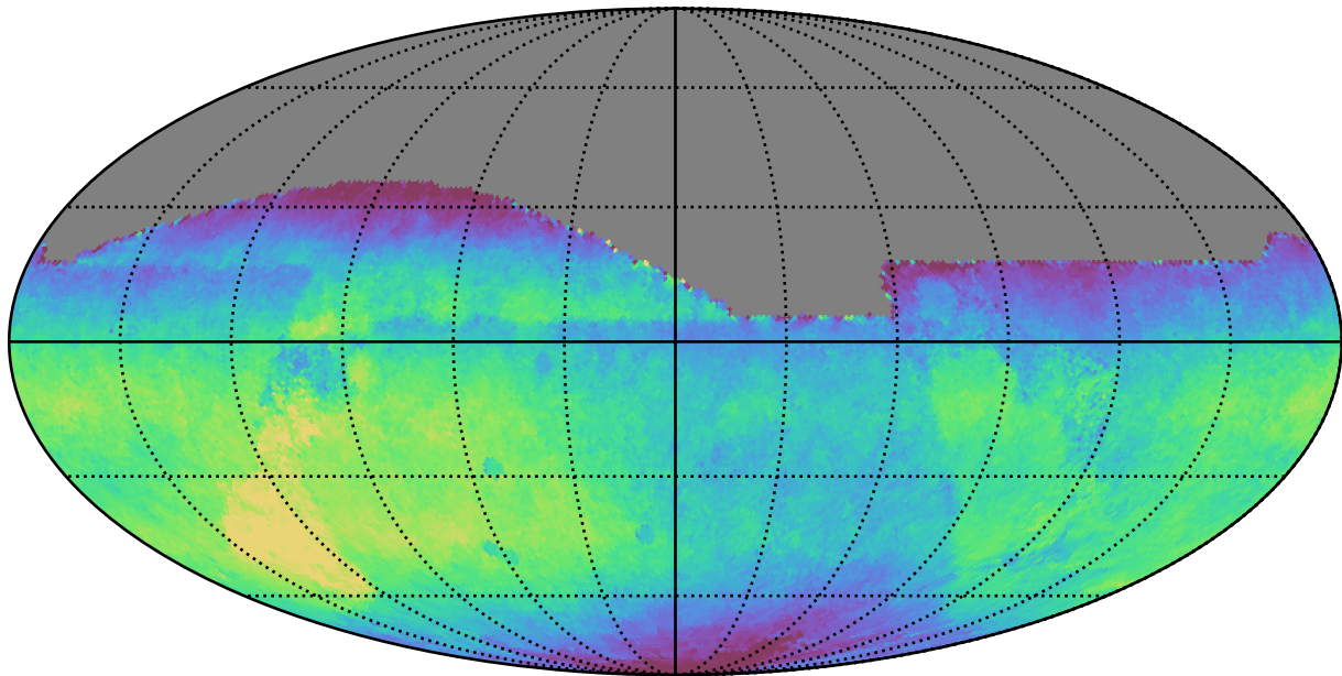
noroll_v3.4_10yrs All sky all bands: Median saturation_mag
