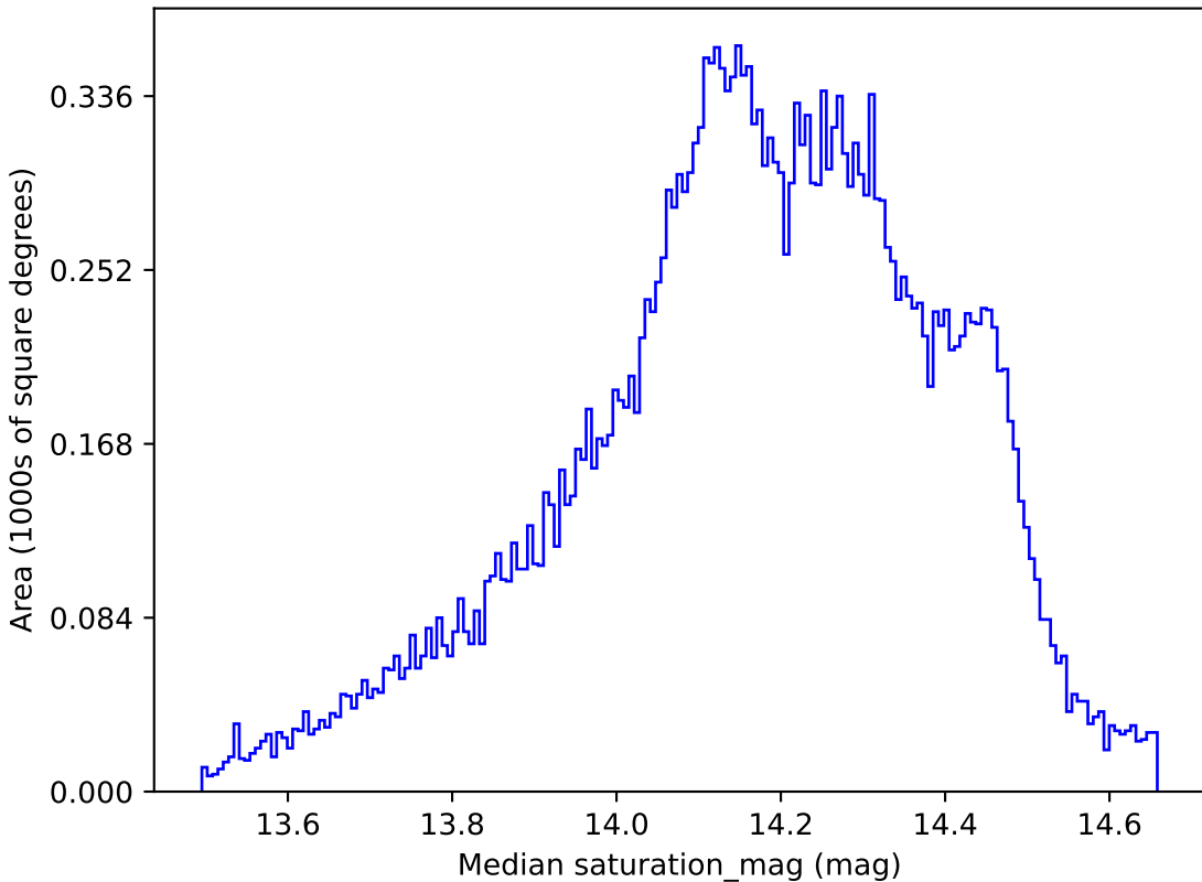
noroll_v3.4_10yrs All sky all bands: Median saturation_mag
