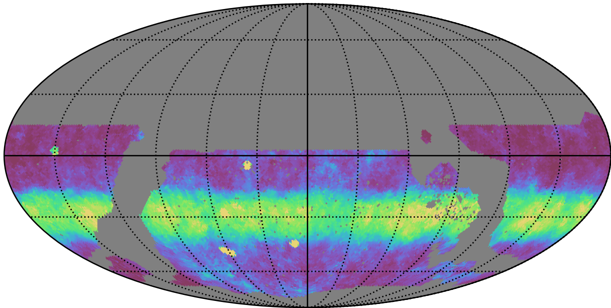
noroll_v3.4_10yrs WFD y band: Median normairmass
