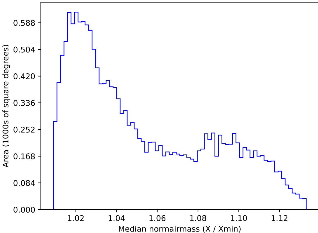
noroll_v3.4_10yrs WFD u band: Median normairmass
