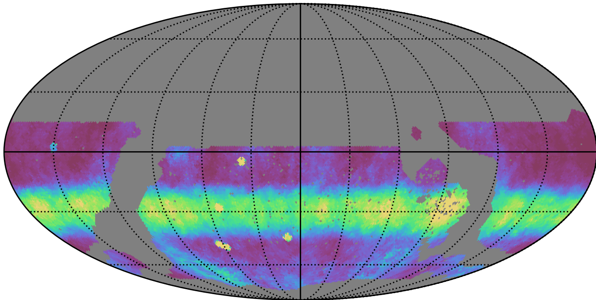
noroll_v3.4_10yrs WFD r band: Median normairmass
