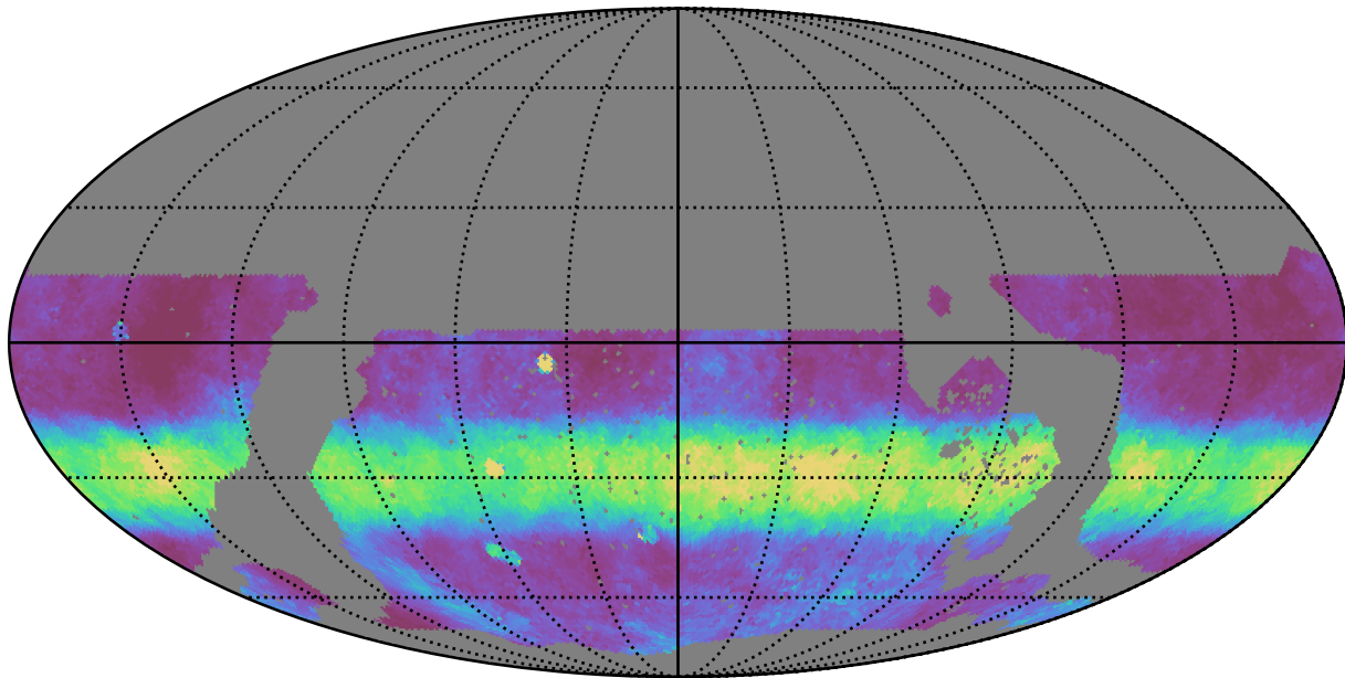
noroll_v3.4_10yrs WFD i band: Median normairmass
