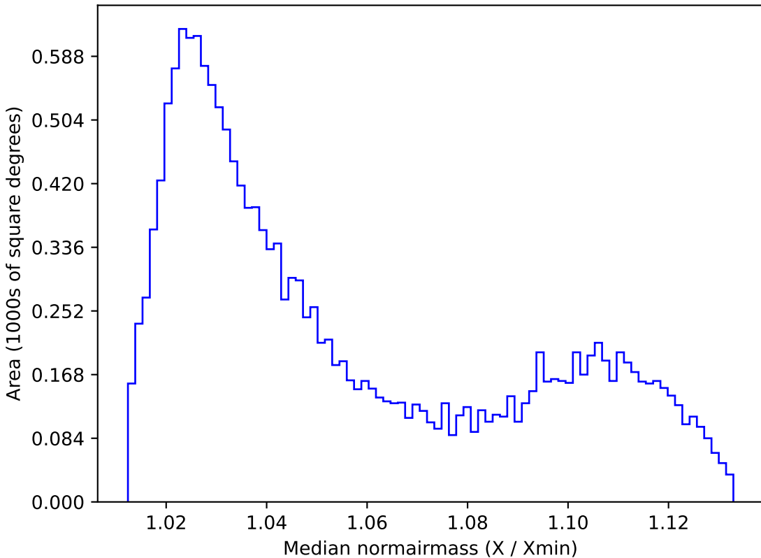
noroll_v3.4_10yrs WFD i band: Median normairmass
