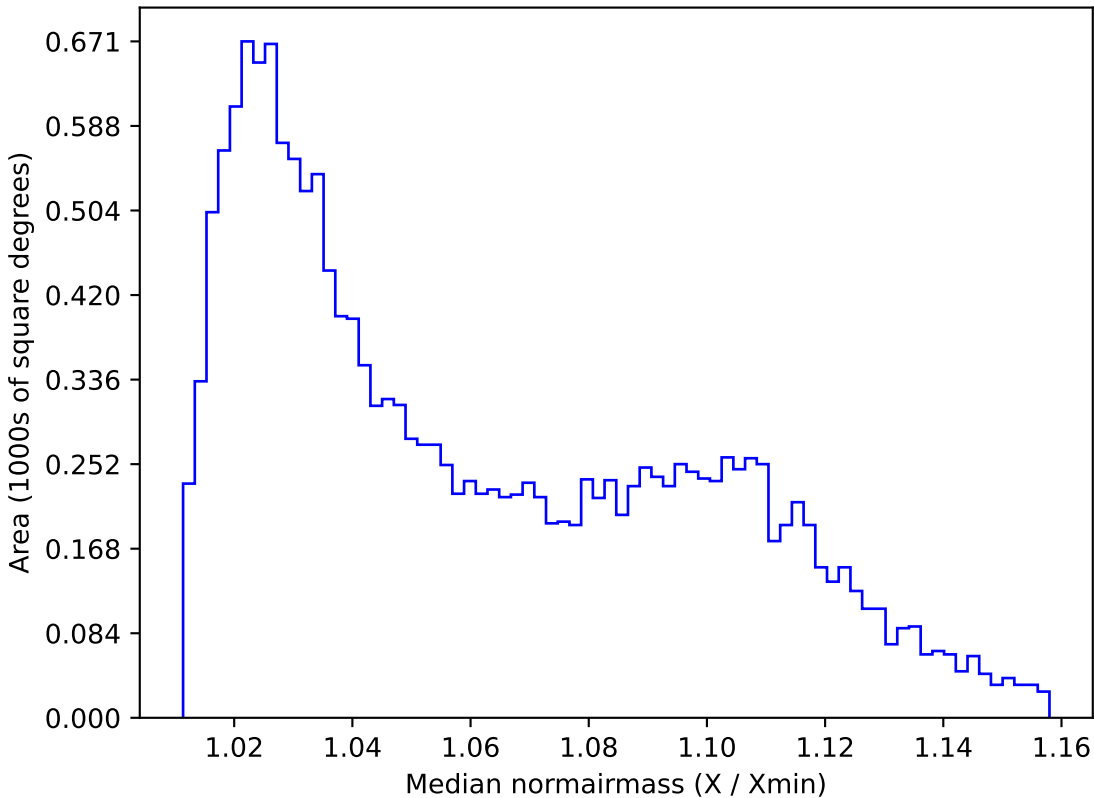
noroll_v3.4_10yrs WFD g band: Median normairmass
