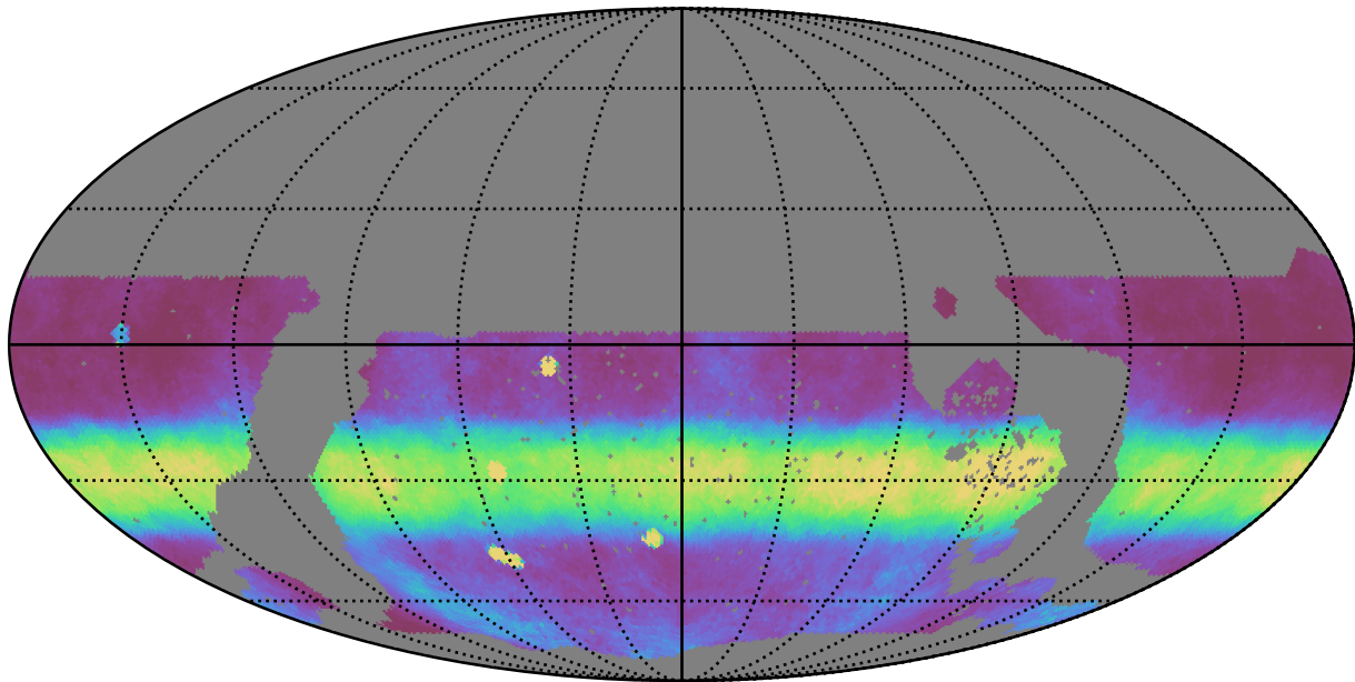
noroll_v3.4_10yrs WFD all bands: Median normairmass
