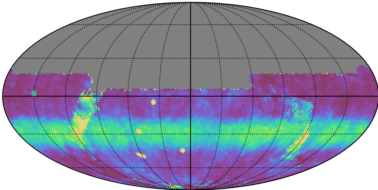
noroll_v3.4_10yrs All sky y band: Median normairmass
