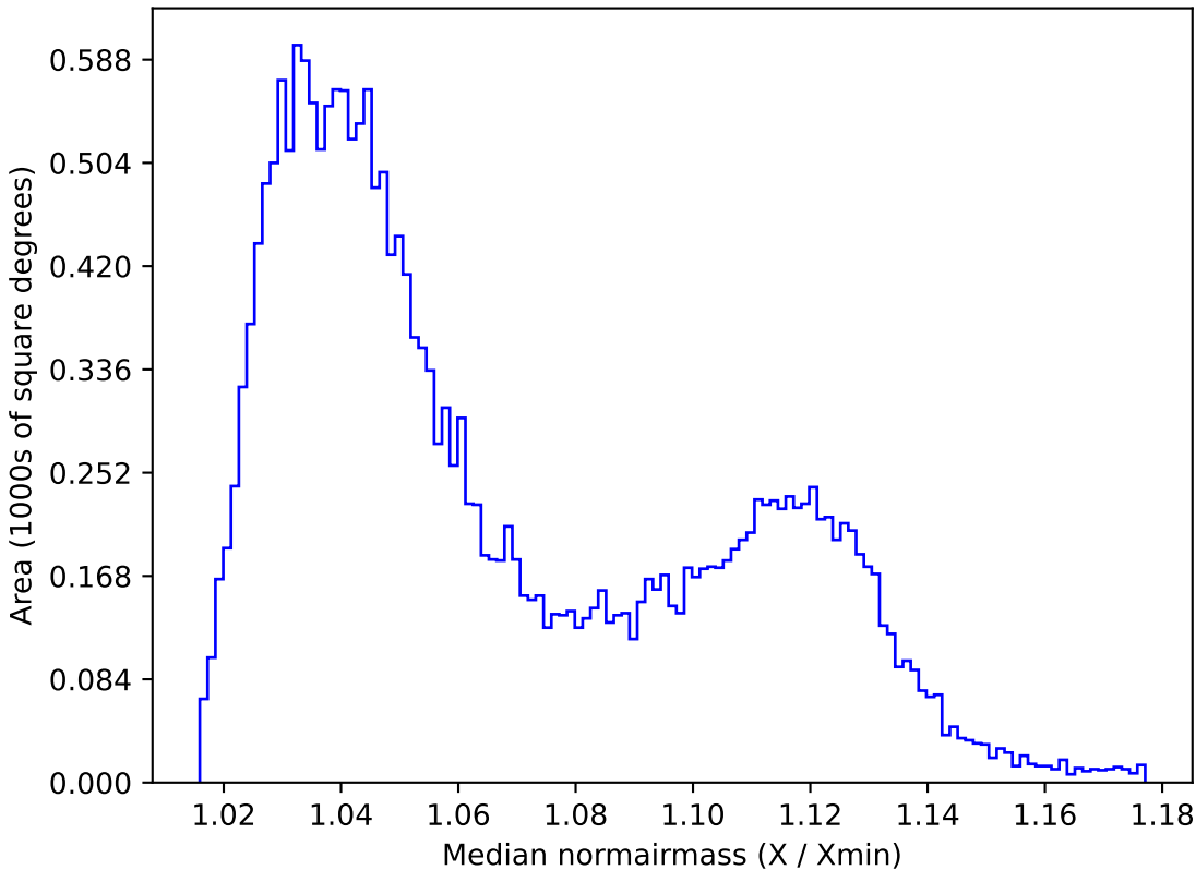
noroll_v3.4_10yrs All sky y band: Median normairmass
