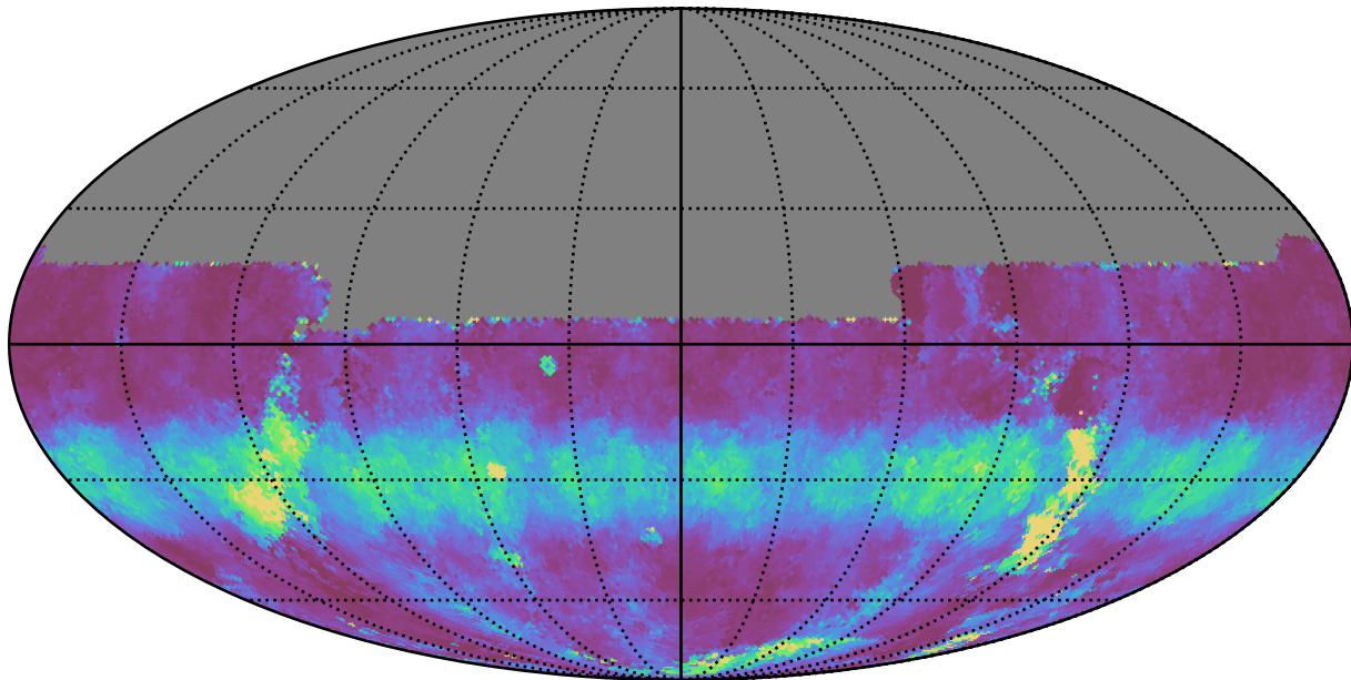
noroll_v3.4_10yrs All sky u band: Median normairmass
