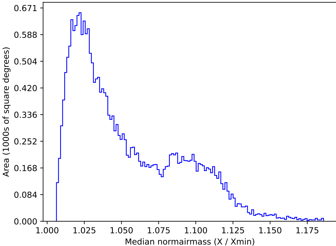
noroll_v3.4_10yrs All sky u band: Median normairmass
