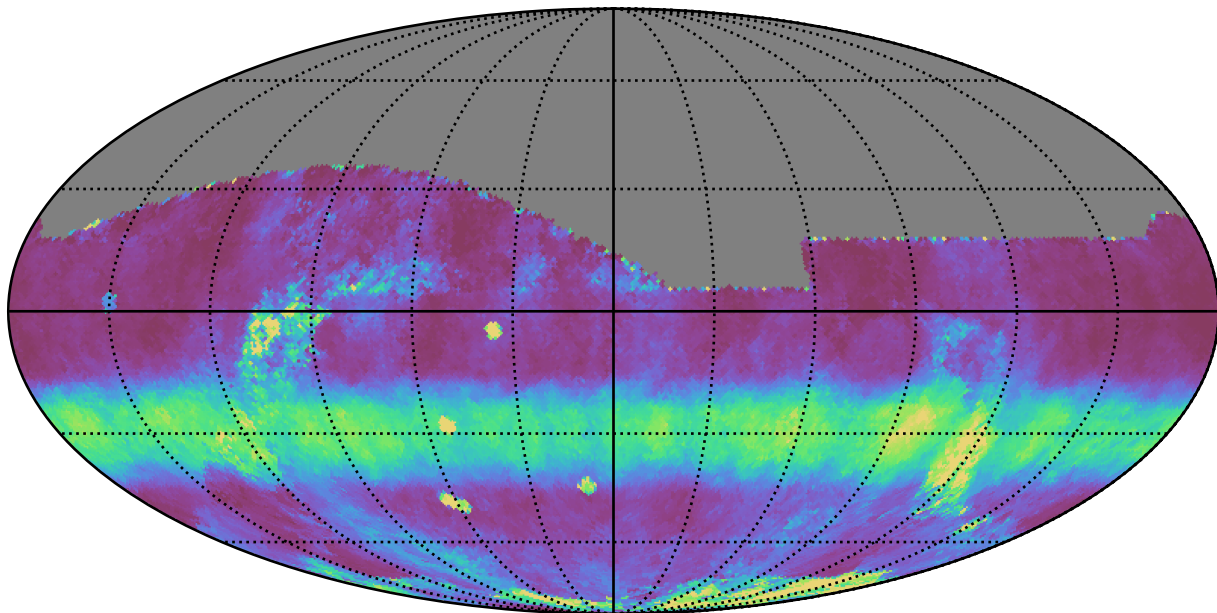
noroll_v3.4_10yrs All sky r band: Median normairmass
