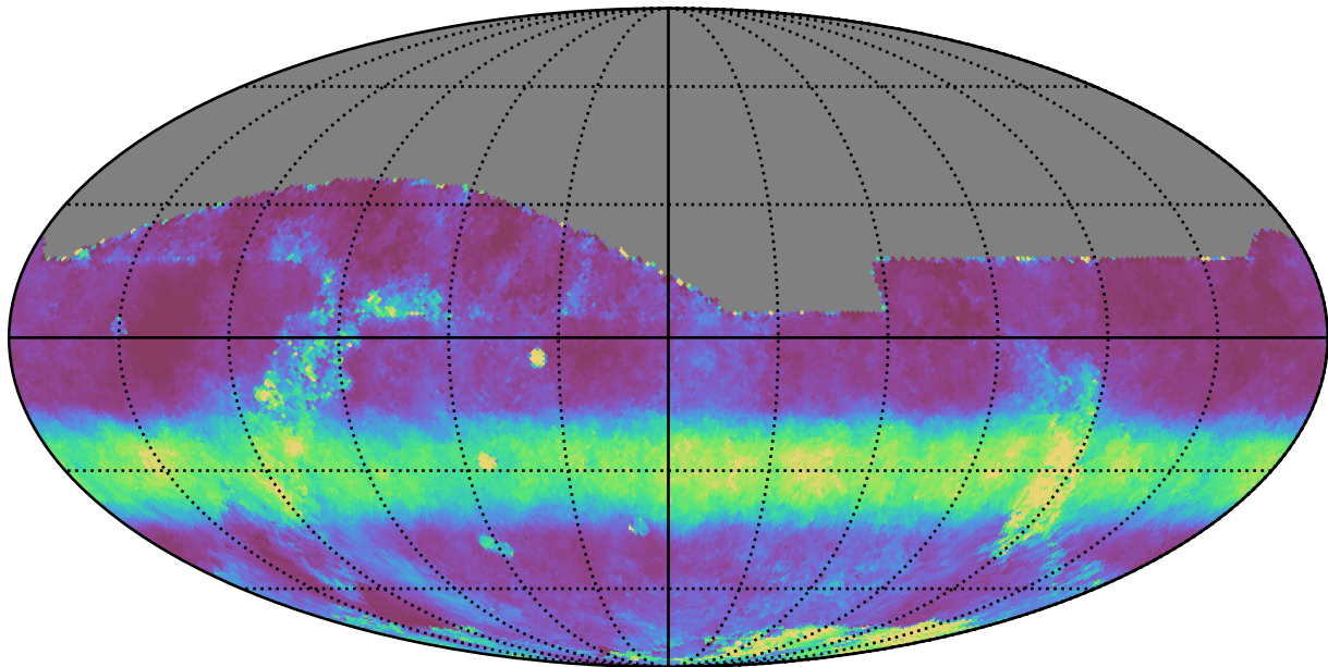
noroll_v3.4_10yrs All sky i band: Median normairmass
