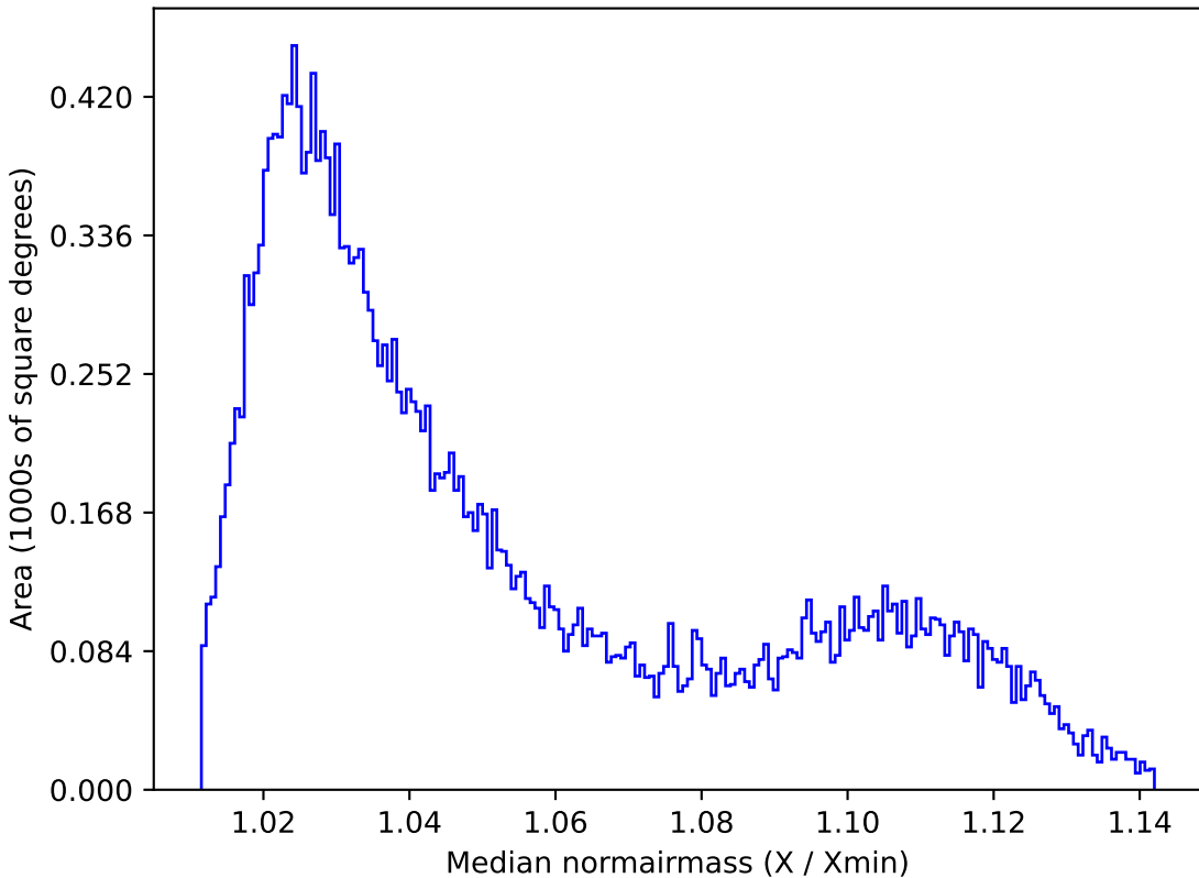
noroll_v3.4_10yrs All sky i band: Median normairmass
