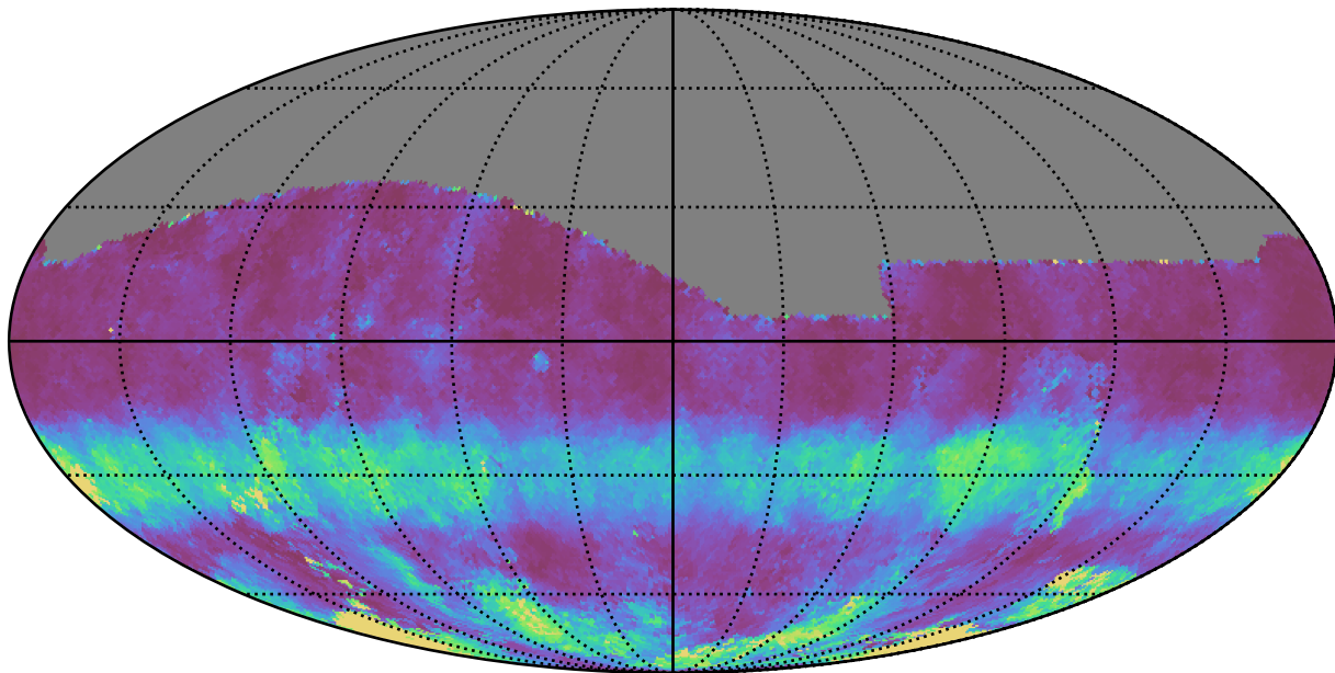
noroll_v3.4_10yrs All sky g band: Median normairmass
