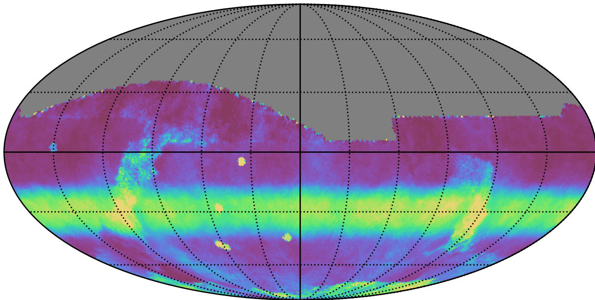
noroll_v3.4_10yrs All sky all bands: Median normairmass
