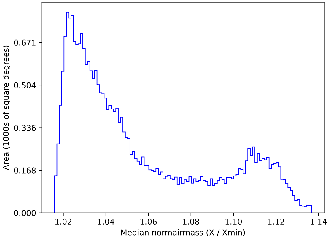
noroll_v3.4_10yrs All sky all bands: Median normairmass
