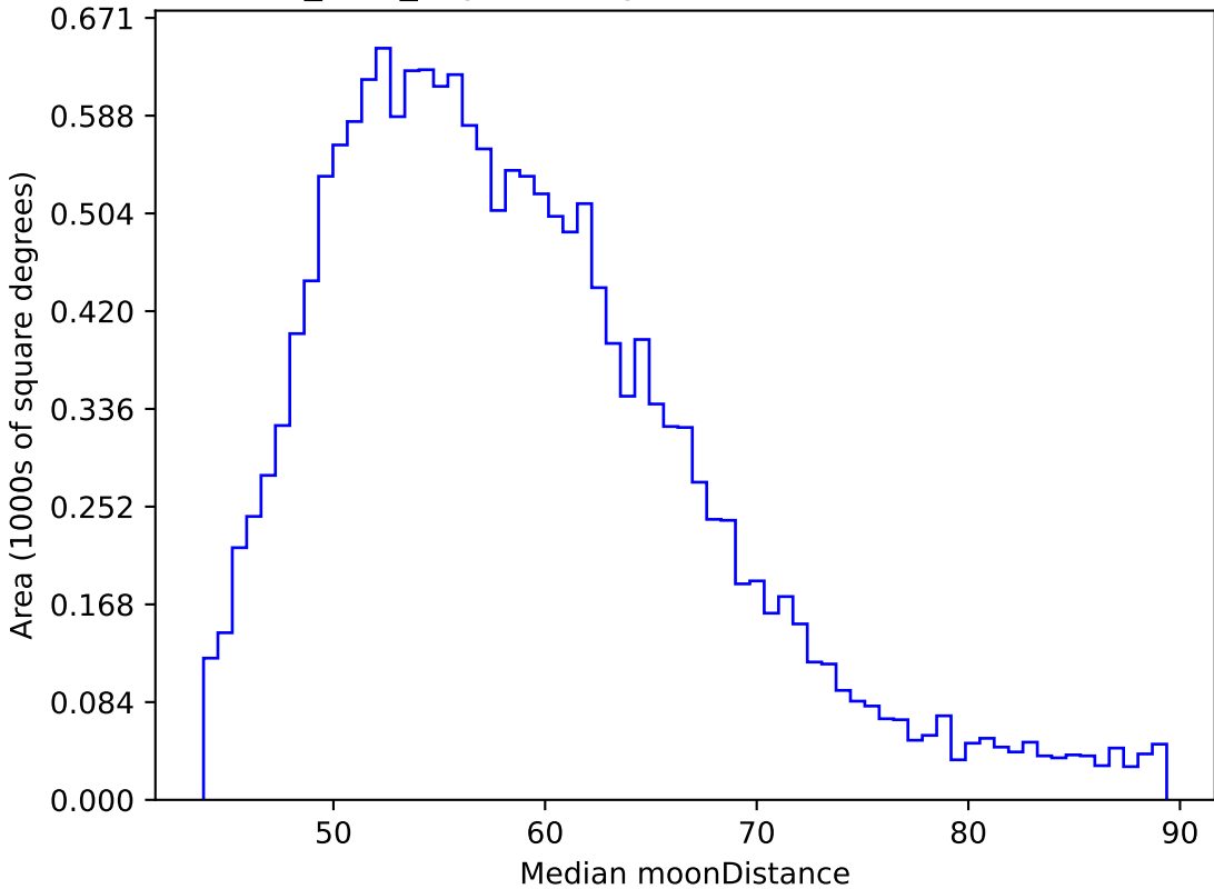
noroll_v3.4_10yrs WFD y band: Median moonDistance
