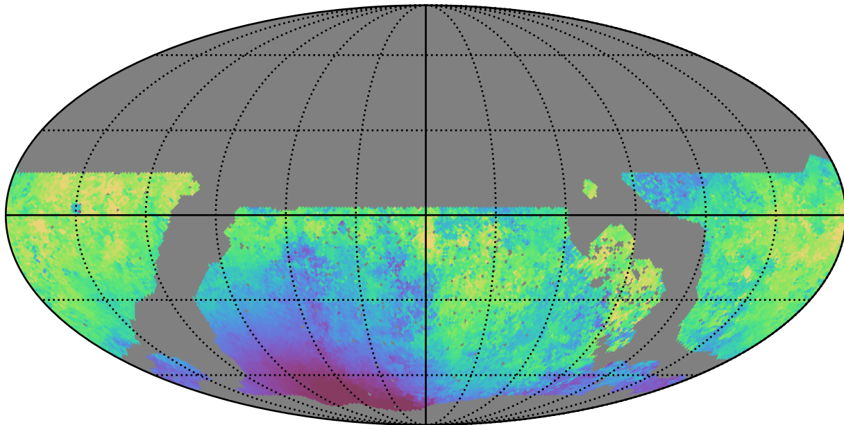
noroll_v3.4_10yrs WFD u band: Median moonDistance
