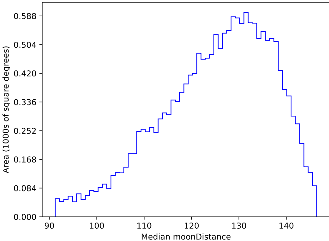
noroll_v3.4_10yrs WFD u band: Median moonDistance
