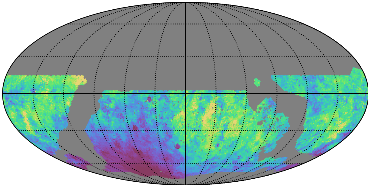
noroll_v3.4_10yrs WFD r band: Median moonDistance
