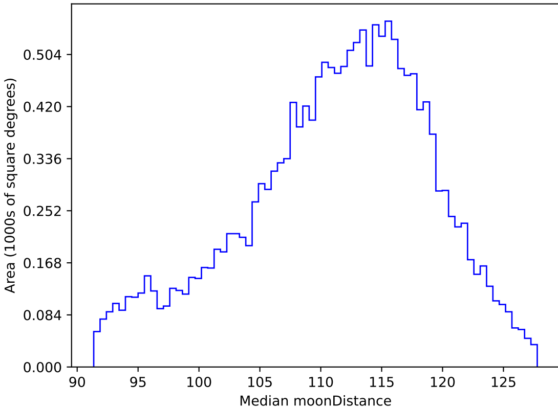
noroll_v3.4_10yrs WFD r band: Median moonDistance
