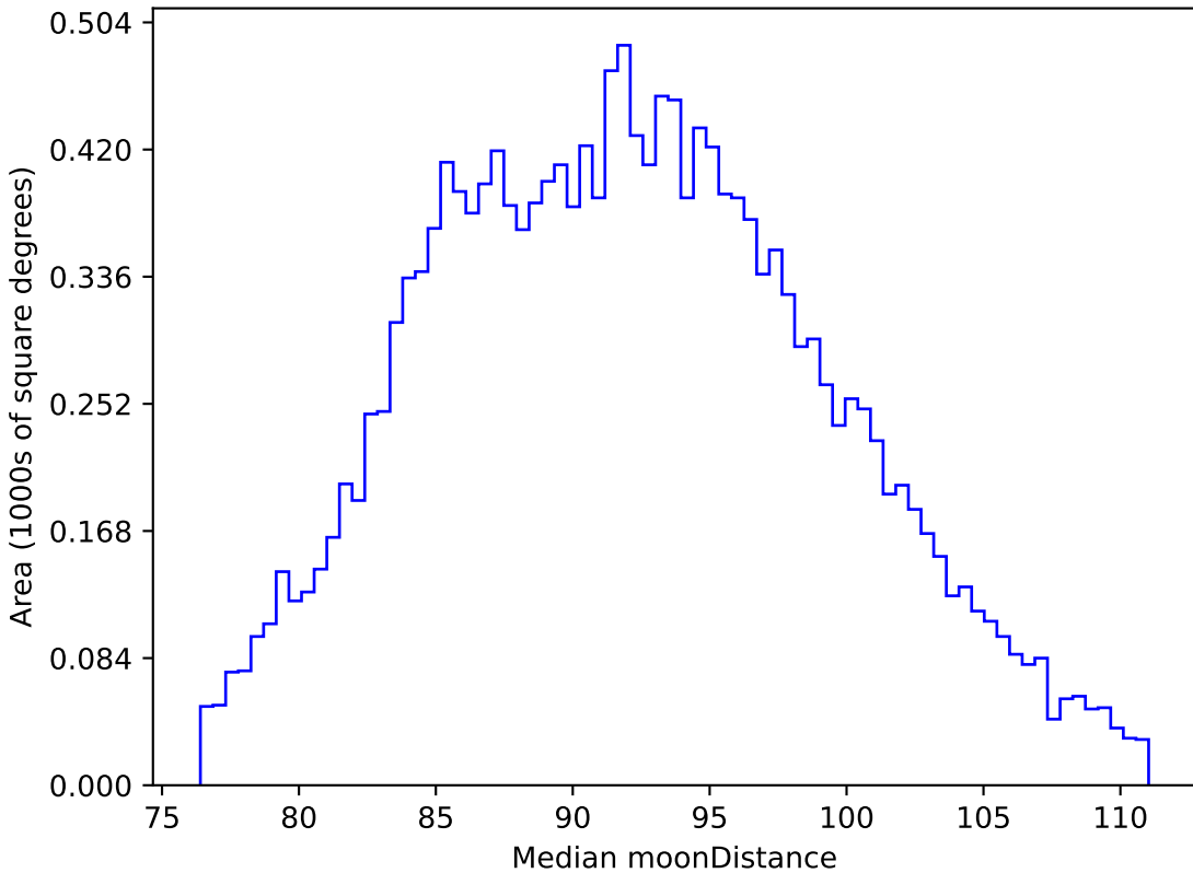
noroll_v3.4_10yrs WFD i band: Median moonDistance
