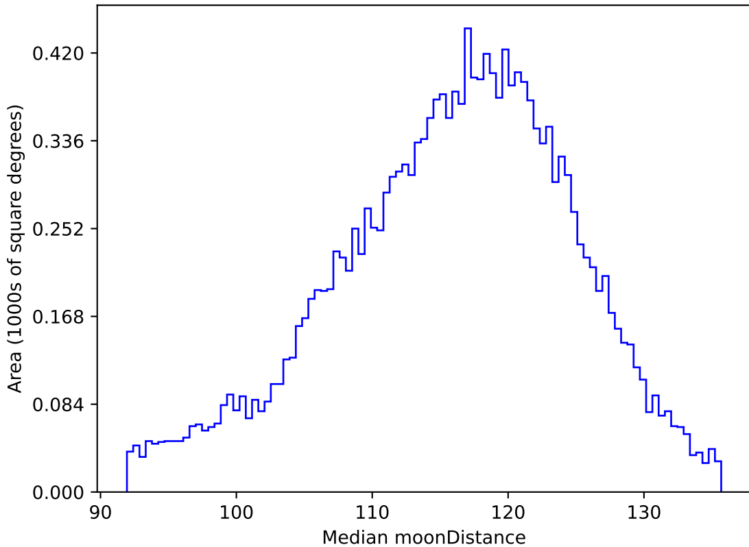
noroll_v3.4_10yrs WFD g band: Median moonDistance
