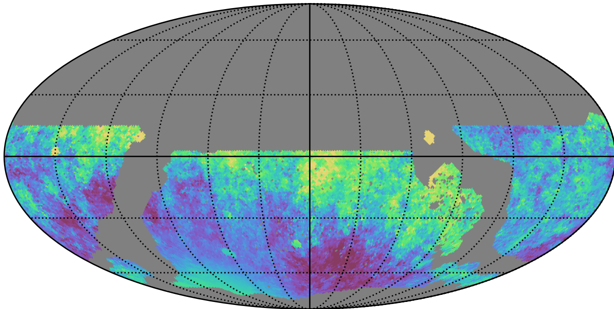
noroll_v3.4_10yrs WFD all bands: Median moonDistance
