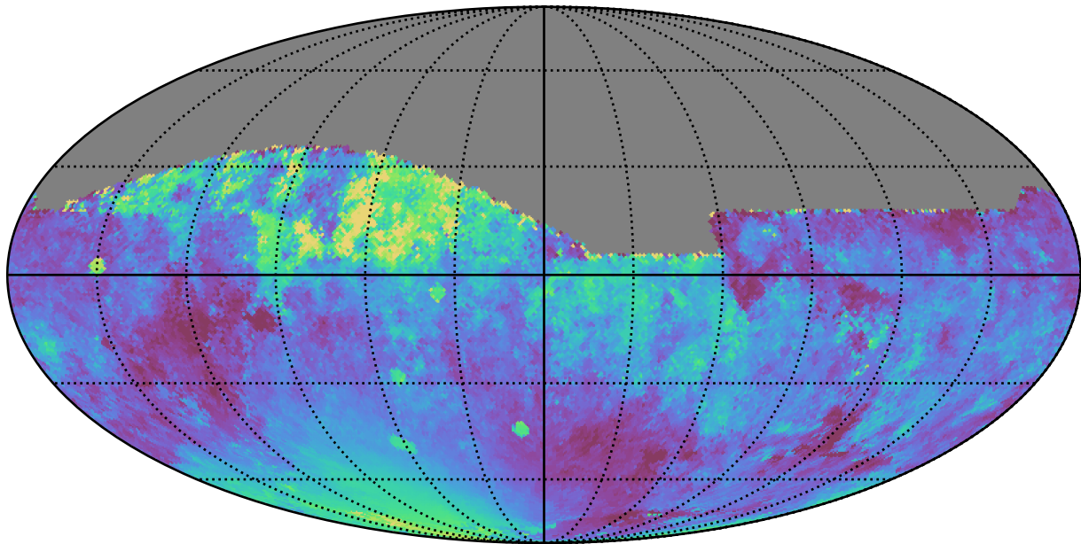
noroll_v3.4_10yrs All sky z band: Median moonDistance
