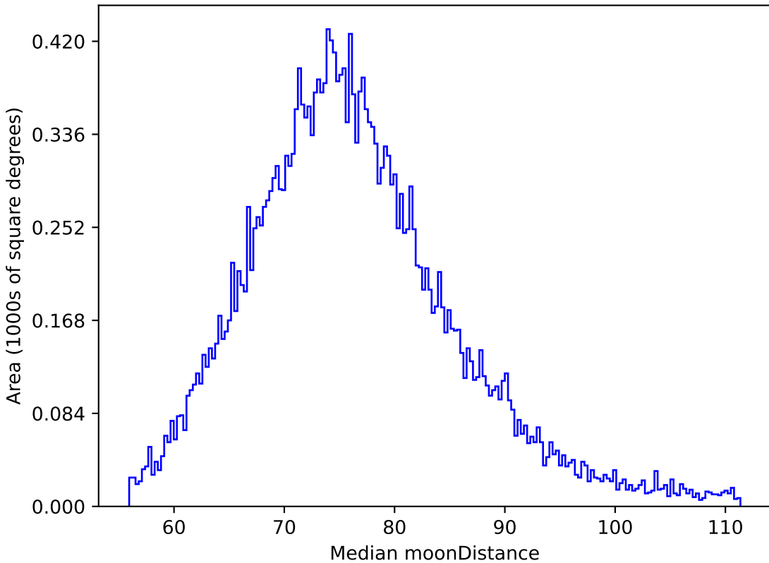
noroll_v3.4_10yrs All sky z band: Median moonDistance
