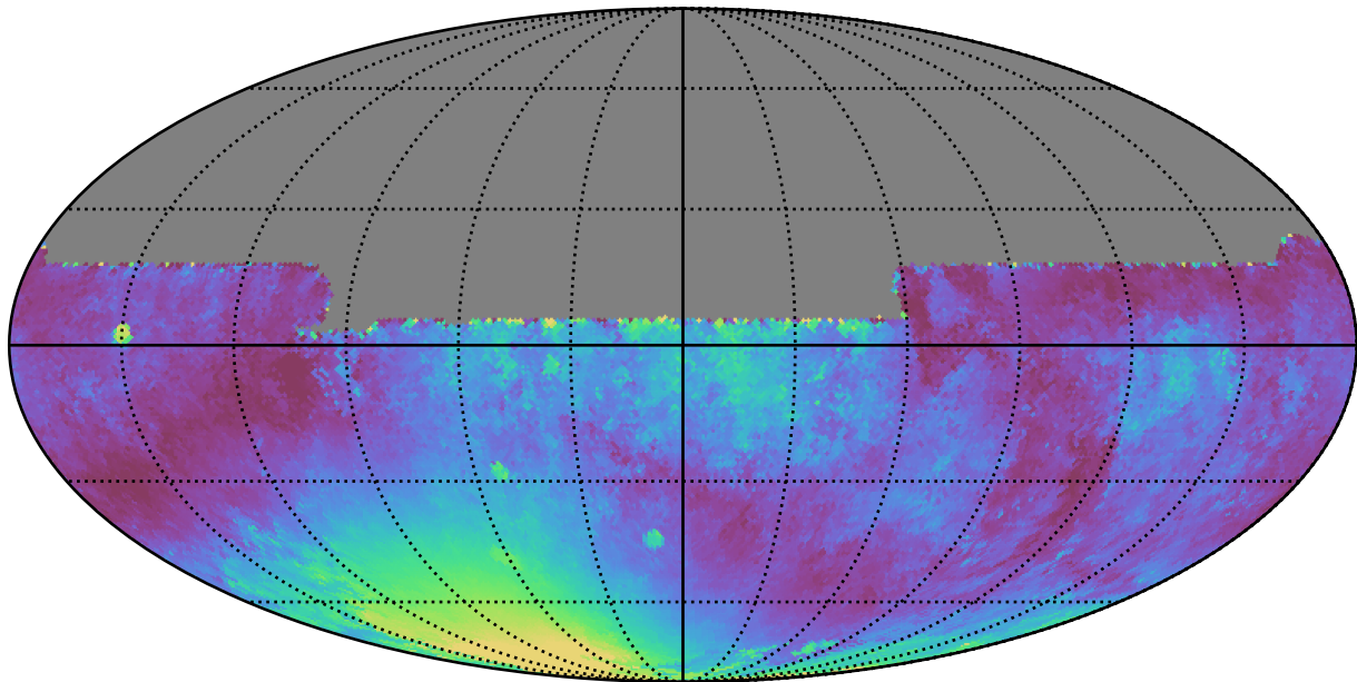
noroll_v3.4_10yrs All sky y band: Median moonDistance
