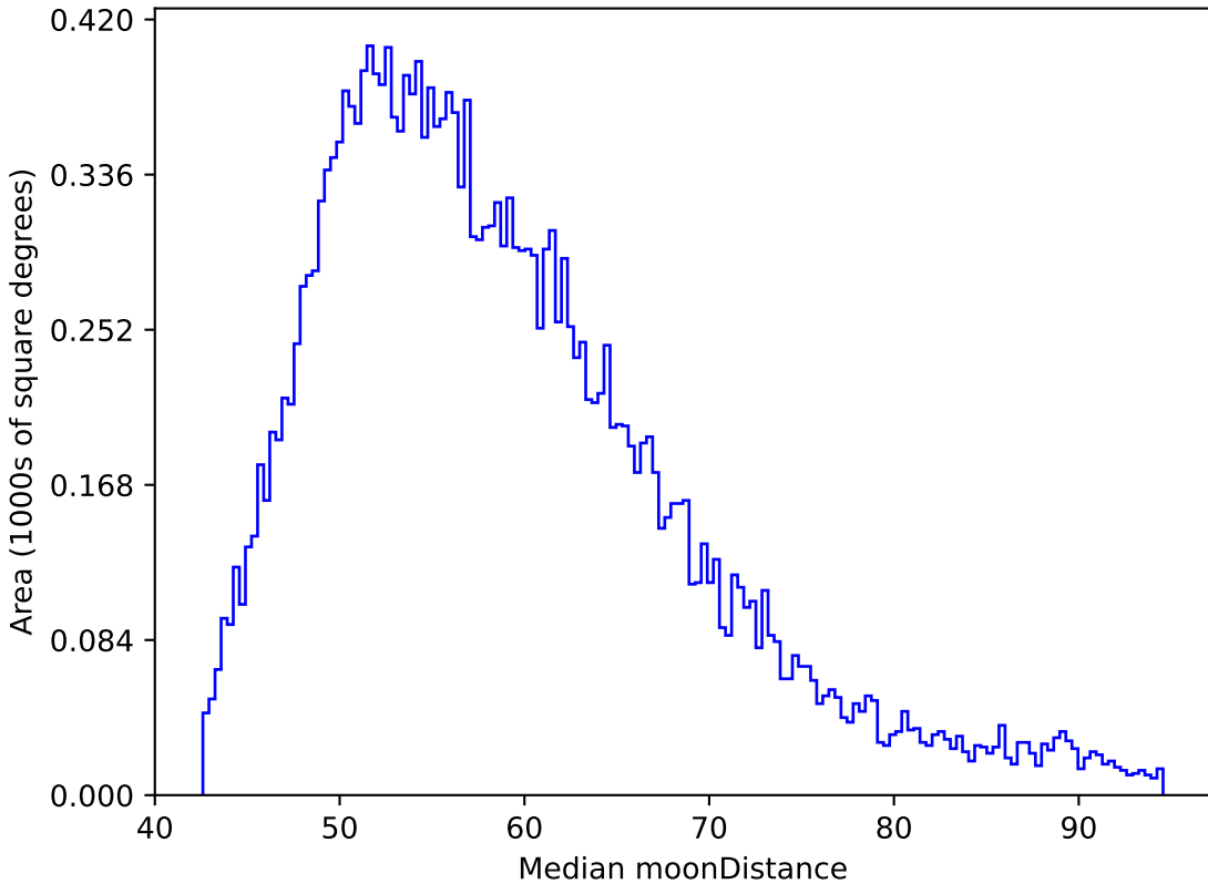
noroll_v3.4_10yrs All sky y band: Median moonDistance
