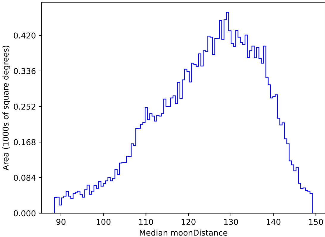
noroll_v3.4_10yrs All sky u band: Median moonDistance
