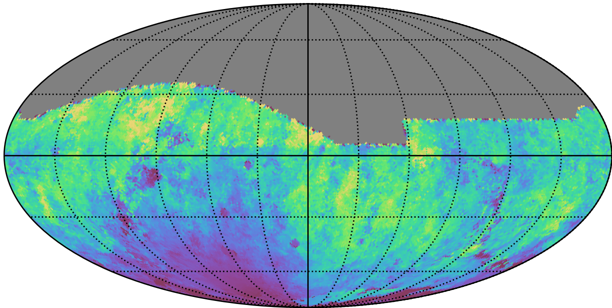
noroll_v3.4_10yrs All sky r band: Median moonDistance
