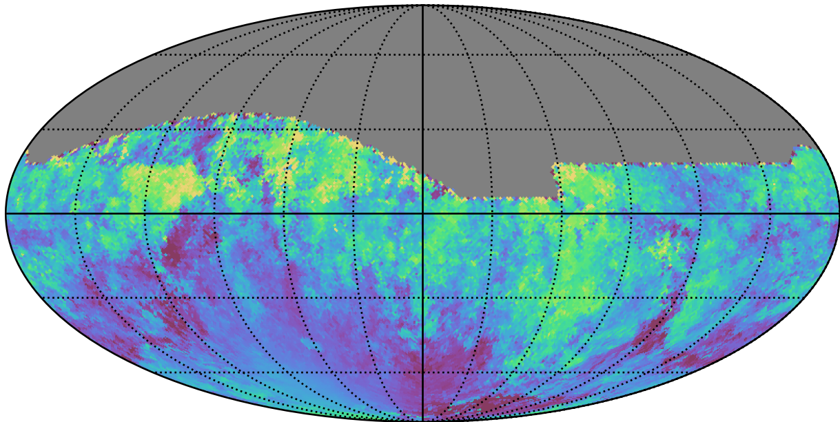
noroll_v3.4_10yrs All sky i band: Median moonDistance
