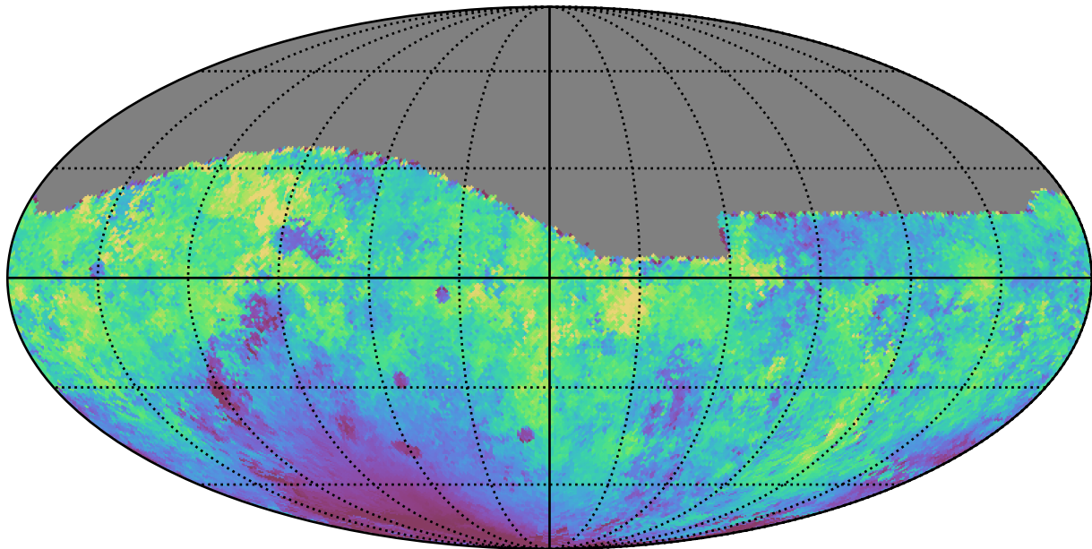
noroll_v3.4_10yrs All sky g band: Median moonDistance
