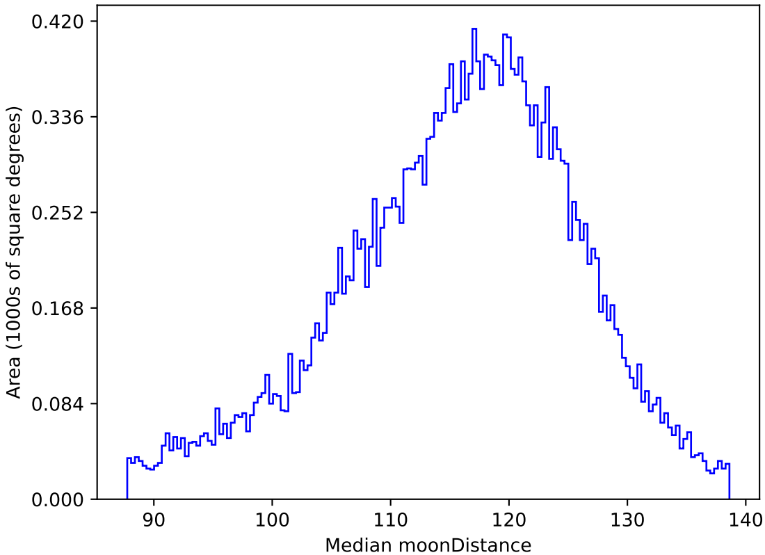
noroll_v3.4_10yrs All sky g band: Median moonDistance
