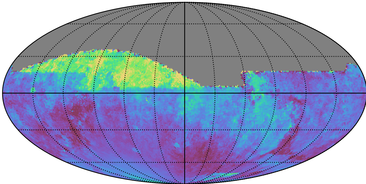
noroll_v3.4_10yrs All sky all bands: Median moonDistance
