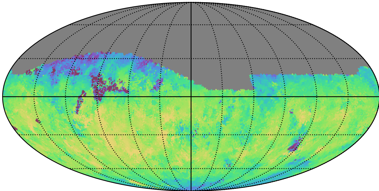
noroll_v3.4_10yrs Yr 1 z band: Median fiveSigmaDepth
