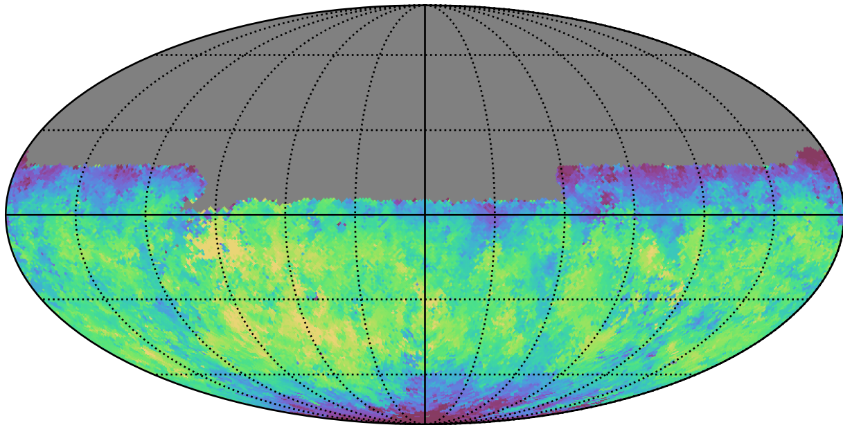
noroll_v3.4_10yrs Yr 1 y band: Median fiveSigmaDepth
