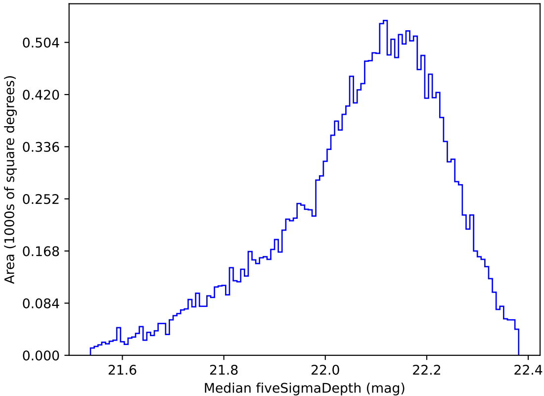
noroll_v3.4_10yrs Yr 1 y band: Median fiveSigmaDepth
