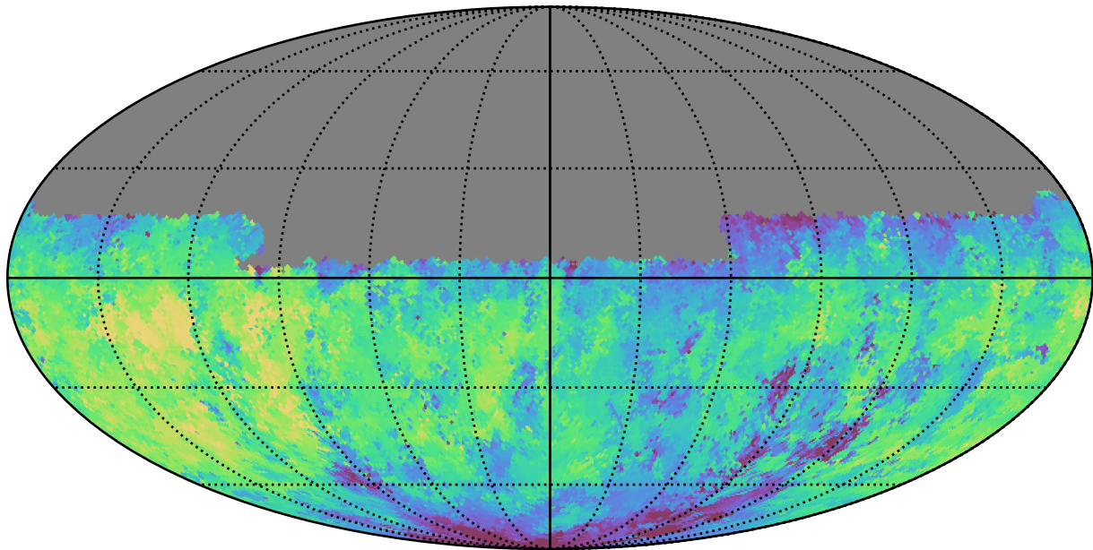
noroll_v3.4_10yrs Yr 1 u band: Median fiveSigmaDepth
