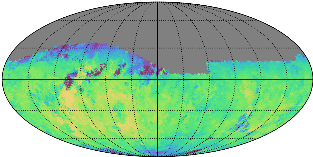
noroll_v3.4_10yrs Yr 1 r band: Median fiveSigmaDepth
