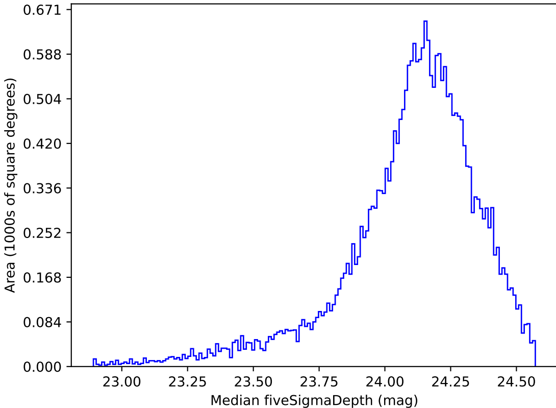
noroll_v3.4_10yrs Yr 1 r band: Median fiveSigmaDepth
